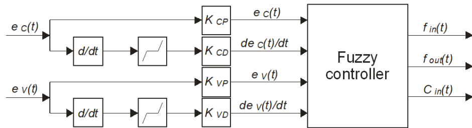
Fig. 6. FLC structure. FLC, fuzzy logic controller
