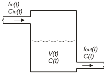
Fig. 1. Scheme of the averaging tank
