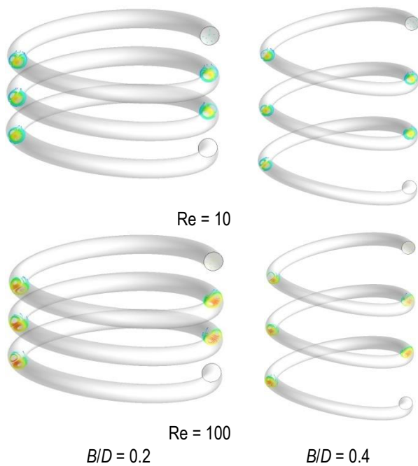
Fig. 9. Streamlines in cross-sections of the angles 180^\circ and -180^\circ in terms of B/D and Re at n = 1 and Ri = 1 ( B , the pitch between the rings; D , diameter of the tube ring. Re , Reynolds number)
