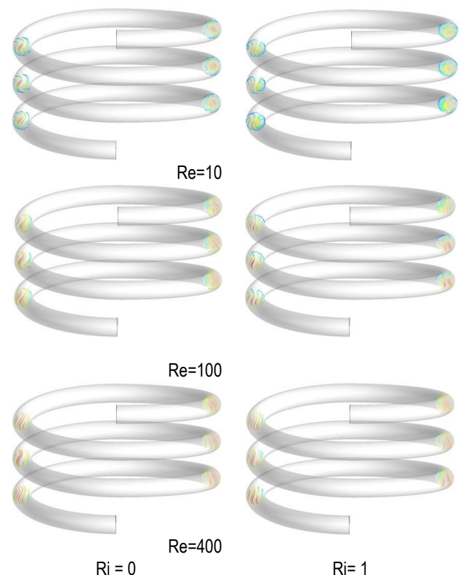
Fig. 5. Streamlines in the cross-sections of the angles 90^\circ and -90^\circ in terms of Re and Ri at n = 1 ( Re , Reynolds number; Ri , Richardson number)
