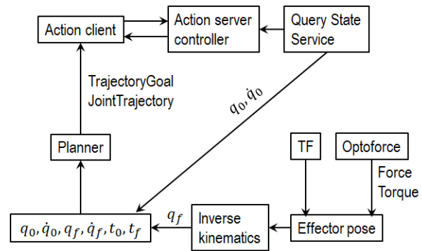
Fig. 8. Block diagram of the proposed system with continuous replanning procedure reacting on sensor readings
