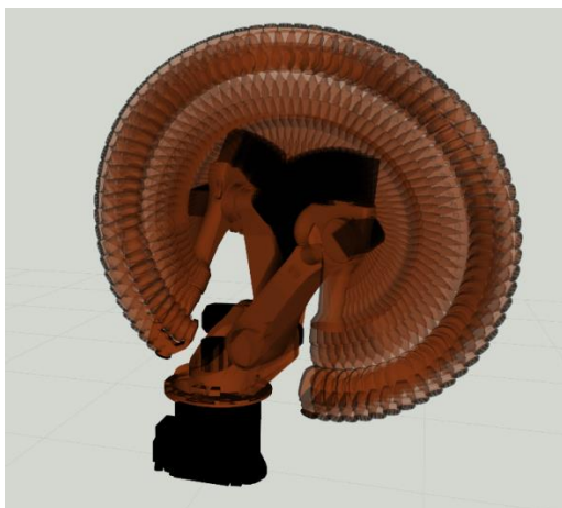
Fig. 10. Displaying a change in the configuration of the arm, which is forced by the need to rotate the first joint by 360° during the execution of Movelt
